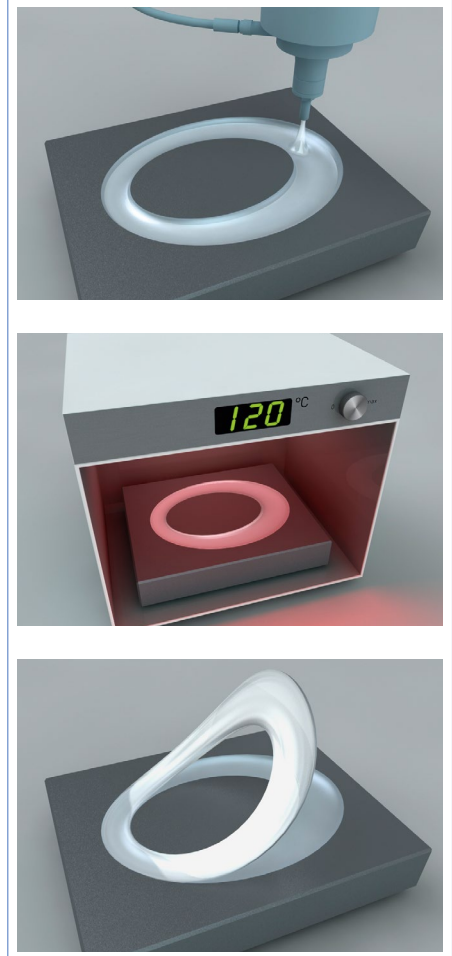
Figure 1: Example of Pelotte Molding Using an ELASTOSIL® P Silicone
