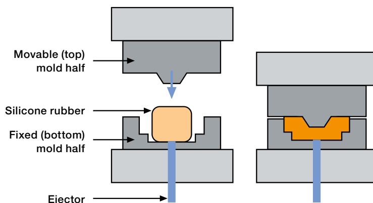
Compression molding
