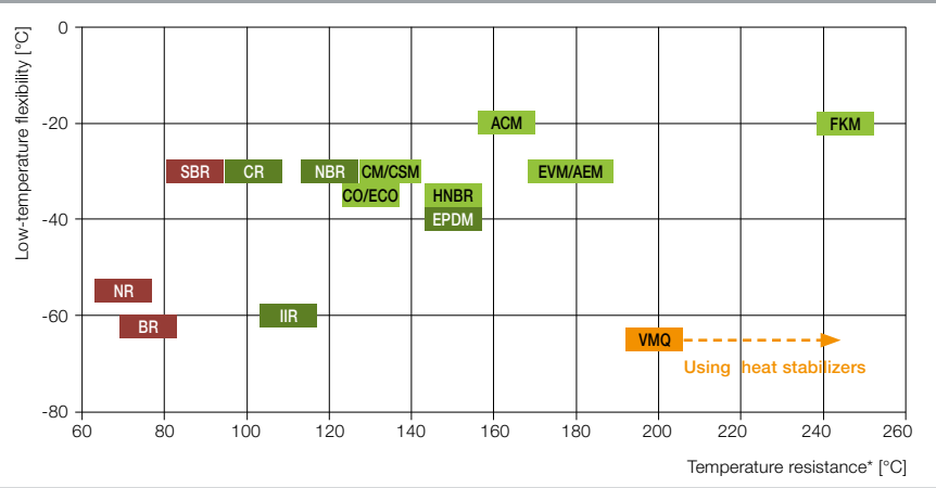
Low-temperature flexibility versus high-temperature resistance
