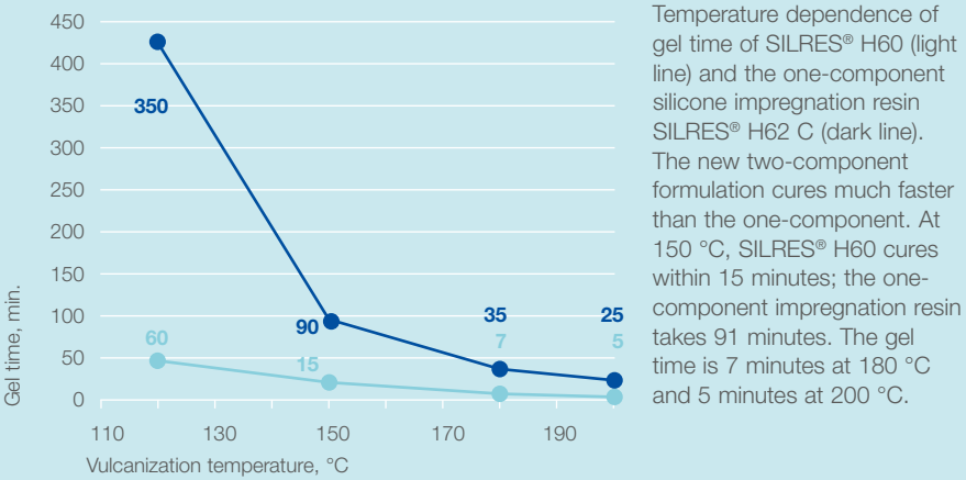
GEL-TIME DEPENDENT ON TEMPERATURE COMPARISON OF SILRES® H62 C and SILRES® H60
