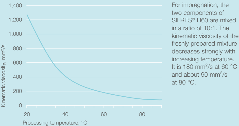
TEMPERATURE DEPENDENCE OF VISCOSITY OF SILRES® H60 A and B mixed in a ratio of 10:1
